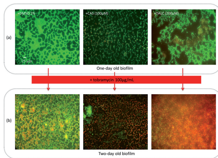
Figure 4. P. aeruginosa biofilm phenotypes and effectiveness of tobramycin treatment in presence of dimethyl sulfoxide (DMSO 1%) or, cassipourol (CAS: 100 \mu M) or oleanolic aldehyde coumarate (OALC: 200 \mu M). (a) After 1 day of incubation, P. aeruginosa fails to form structured confluent aggregate in presence of CAS or OALC as compared to DMSO treatment. (b) CAS and OALC considerably increase the susceptibility of P. aeruginosa to tobramycin (100 \mu g/mL), as shown by the increased proportion of dead cells compared with DMSO. Similar results are observed when tobramycin is added simultaneously with CAS or OALC to one-day old untreated biofilms. The bacterial viability was assessed by staining the cells with SYTO-9 (green areas zones—live living bacteria) and propidium iodide (red areas zones—dead bacteria) furnished in the LIVE/DEAD BacLight kit. Cells were visualized using a LeicaDMIRE2 inverted fluorescence microscope using equipped with a 40 \times objective lens and colored images were assembled using Adobe Photoshop.
