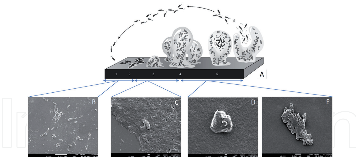
Figure 1. Sketch of the different steps of a biofilm development (A) [15]. Several representative scanning electron microscopy (SEM-JEOL JSM-7200F) images of the P. aeruginosa biofilm at different steps of development and with different magnifications (B = reversible and irreversible stages at 8 h growth, C = microcolonies stage at 30 h growth, D = mature biofilm stage at 120 h growth, and E = dispersion stage at 144 h growth). P. aeruginosa PAO1 colonies were grown at 37°C with Centers for Disease Control and Prevention (CDC) biofilm reactor (biosurface technologies, MT) on tryptone soy broth (TSB).
