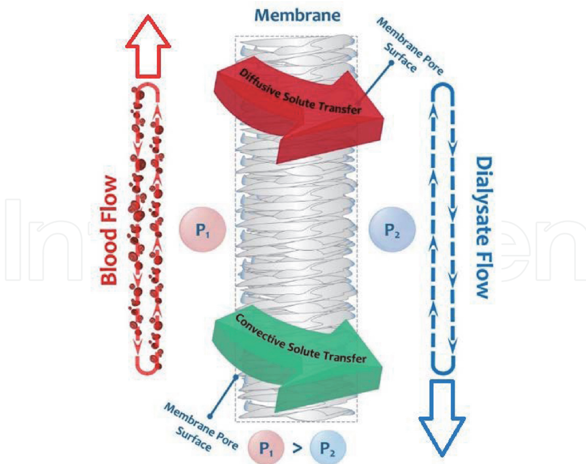
Figure 1. Schematic diagram of a membrane in hemodialysis process: The left side describes the blood side of the membrane and the right side shows the dialysate side of the process. P_1 and P_2 describe pressure within the blood and dialysate side, respectively. Due to the difference in chemical potential, solutes in blood move through the membrane to the dialysate side.
