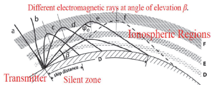
Figure 8. Simple scheme of an ionospheric radio link.
