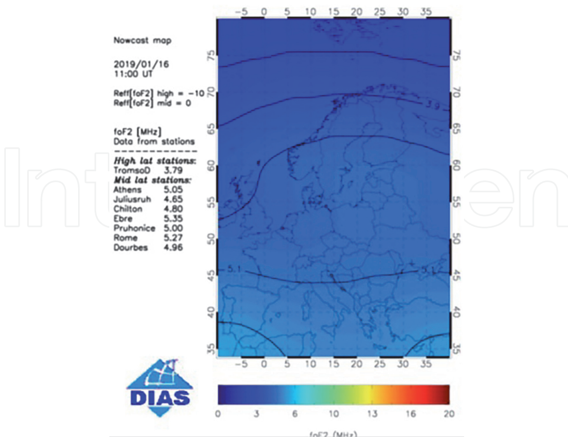
Figure 7. An example of the foF2 nowcast map predicted by SIRMUP model in 16 January 2019 at 11:00 UT for DIAS ( http://www.iono.noa.gr/Dias/ ).
