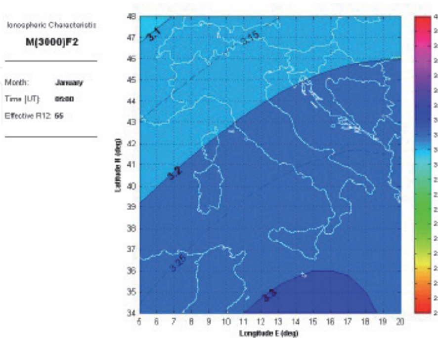
Figure 11. Examples of foF2 and M(3000)F2 nowcast maps predicted by SIRMUP model for the Central Mediterranean area at two different hours and effective solar activity index R_{12,eff} .
