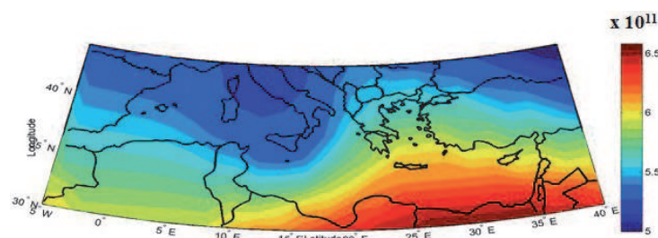
Figure 14. Map of the ionospheric electron density in el/m^3 at the fixed height of 201 km obtained by the IRI-SIRMUP-P procedure for a given epoch.
