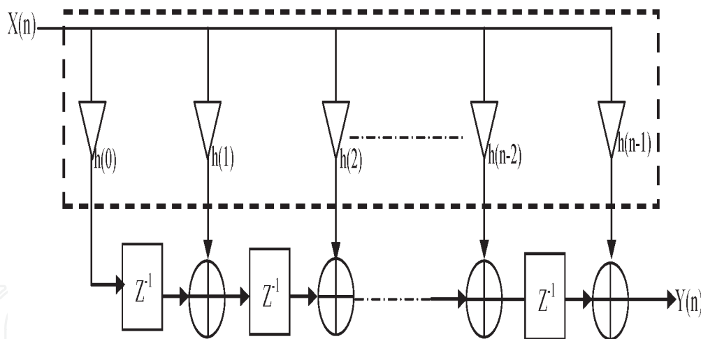
Figure 1. Transposed direct form FIR filter architecture.
