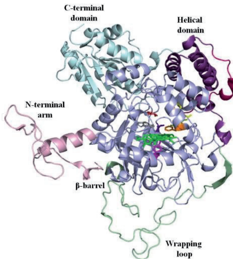
Figure 2. Schematic drawing of the polypeptide chain and elements of secondary structure in a S. thermophilum catalase subunit. The heme is colored green, Tyr369 magenta, His82 gray, Asn155 purple blue, Val123 red, Phe160 lemon, Phe161 yellow, and Phe168 orange. This figure is taken from the report of Yuzugullu et al. [17].
