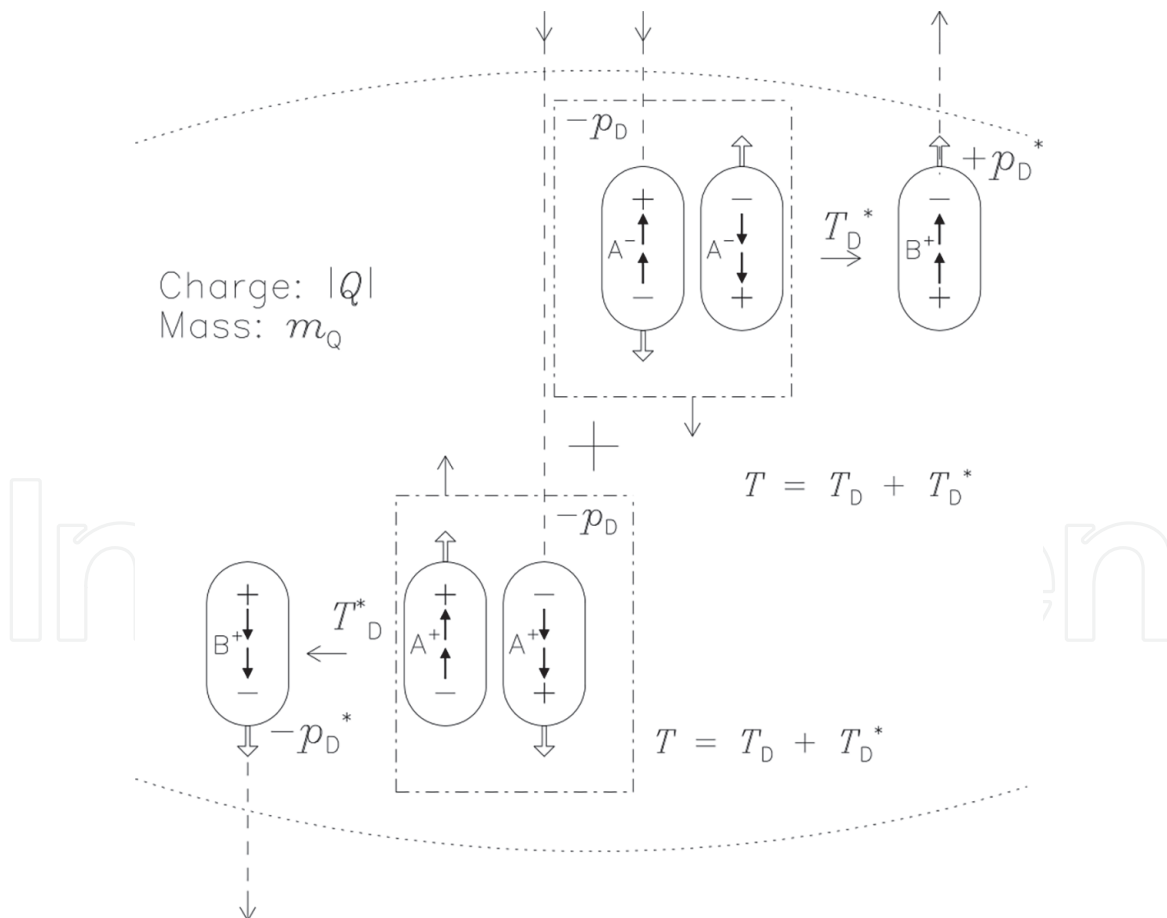
Figure 4. Virtual dipoles emitted by a charge +|Q| (with mass m_Q ) interact with real dipoles, A^+ and A^- arriving with a momentum -p_D , each. On the left, a dipole A^+ combines in the lower dashed-dotted box with virtual dipole A^+ in its destruction phase and liberates dipole B^+ . No momentum will be transferred to the central charge with p_D = p_D^* . The other types of interaction—called direct interaction, in contrast to the indirect one on the left—also require two virtual dipoles, one of them combines in its creation phase with dipole A^- (in the upper box with dashed-dotted boundaries), and the other one is liberated by the excess energy of the annihilation. The central charge received a momentum of -(p_D + p_D^*) = -2p_D . No spin reversal has been assumed in both cases.
