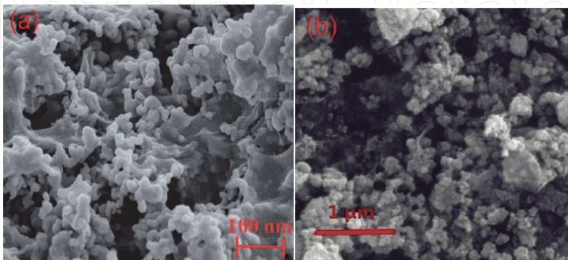
Figure 1. SEM image of hydrothermally grown SnO 2 nanoparticles and rGO composites reported by (a) Zhang et al. [33] and (b) Peng et al. [41].
