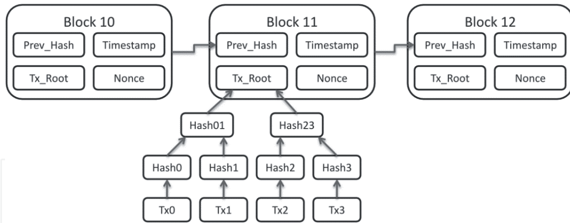
Figure 2. Merkle tree.
