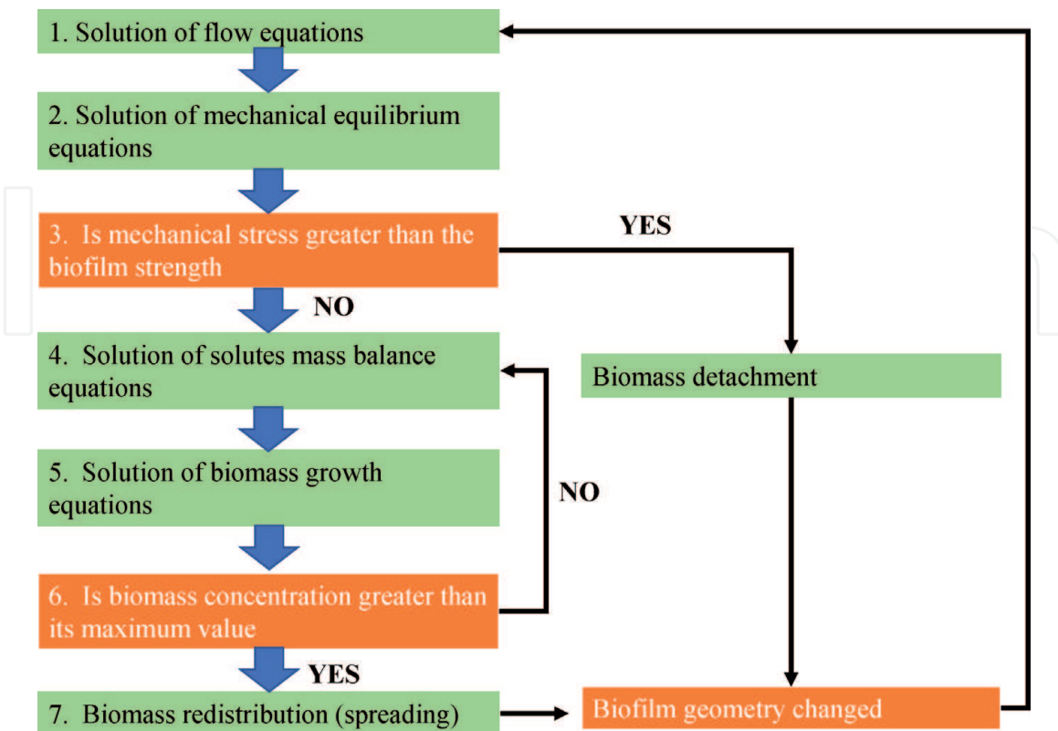
Figure 1. Algorithm steps for the biofilm model including substrate convection, substrate diffusion, substrate reaction, biomass growth, and biofilm detachment.
