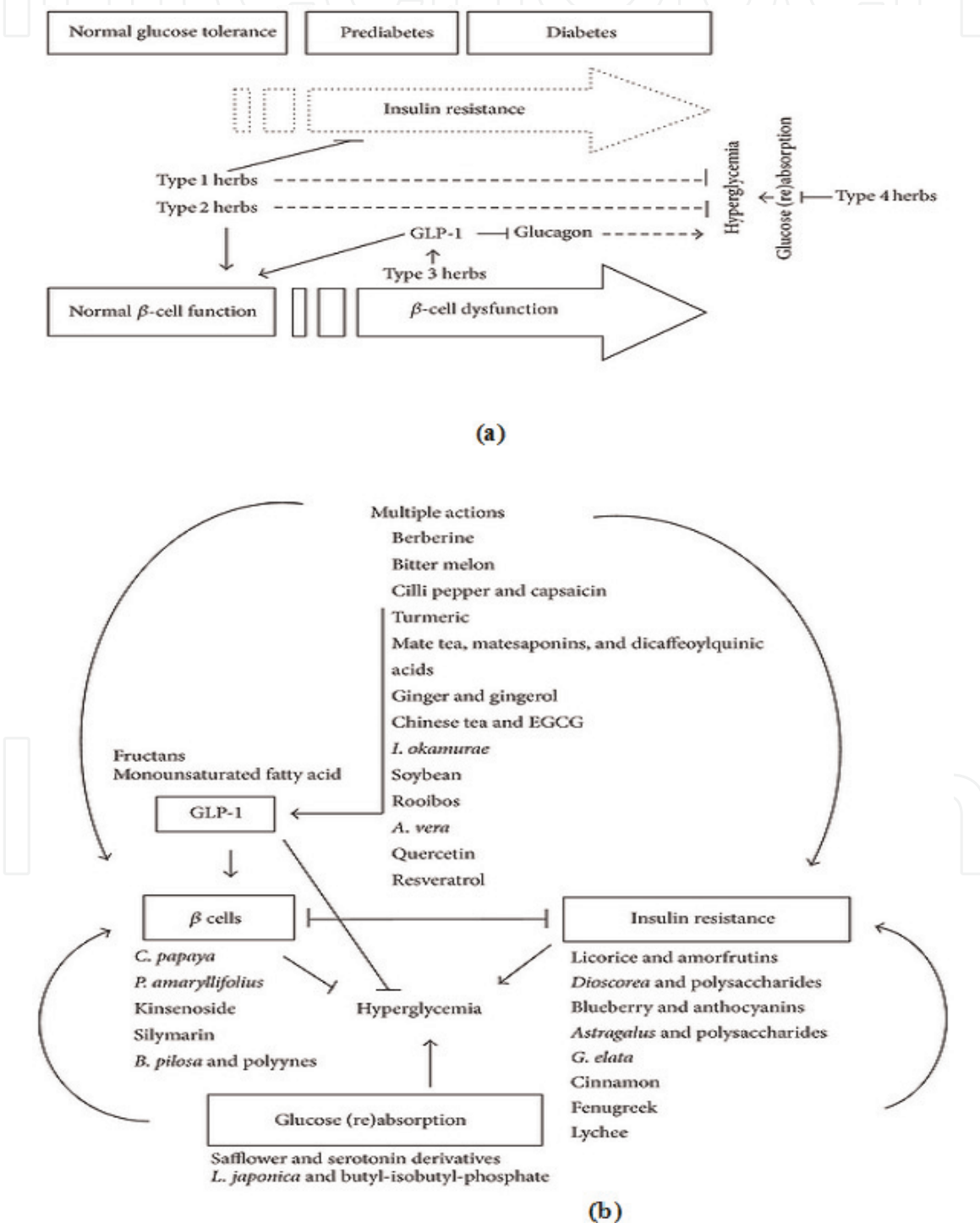
Figure 6. Mechanisms underlying herbal therapies using antidiabetic plants and phytochemicals. (a) Different types of medicinal herbs can be classified based on their modes of action such as insulin resistance (type 1 herbs), \beta -cell function (type 2 herbs), and GLP-1 (type 3 herbs) and glucose (re) absorption (type 4 herbs), (b) The selected.
