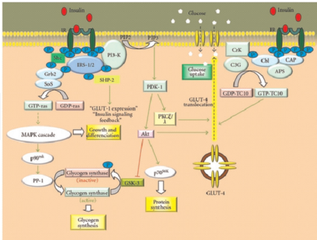
Figure 5. Summary of the main insulin signaling pathways. GLUT-1 and -4: Glucose transporter-1 and -4; Grb-2: Growth receptor binding-2; GSK-3: Glycogen synthase kinase-3; IR: Insulin receptor; IRS-1 and -2: Insulin receptor substrate-1 and -2; MAPK: Mitogen-activated protein kinase; PDK-1: Phosphoinositide-dependent kinase-1; PIP2: Phosphatidyl-inositol diphosphate; PI3: Phosphatidyl-inositol triphosphate; P: Phosphate; PKC: Protein kinase C; PP-1: Phosphoprotein phosphatase-1; p70 S6K : Protein 70 S6 kinase; p90 RSK : Protein 90 ribosomal S6 kinase; Shc: Src homology collagen; SHP-2: Phosphatase with Src homology 2 domain; SoS: Son of Sevenless.
