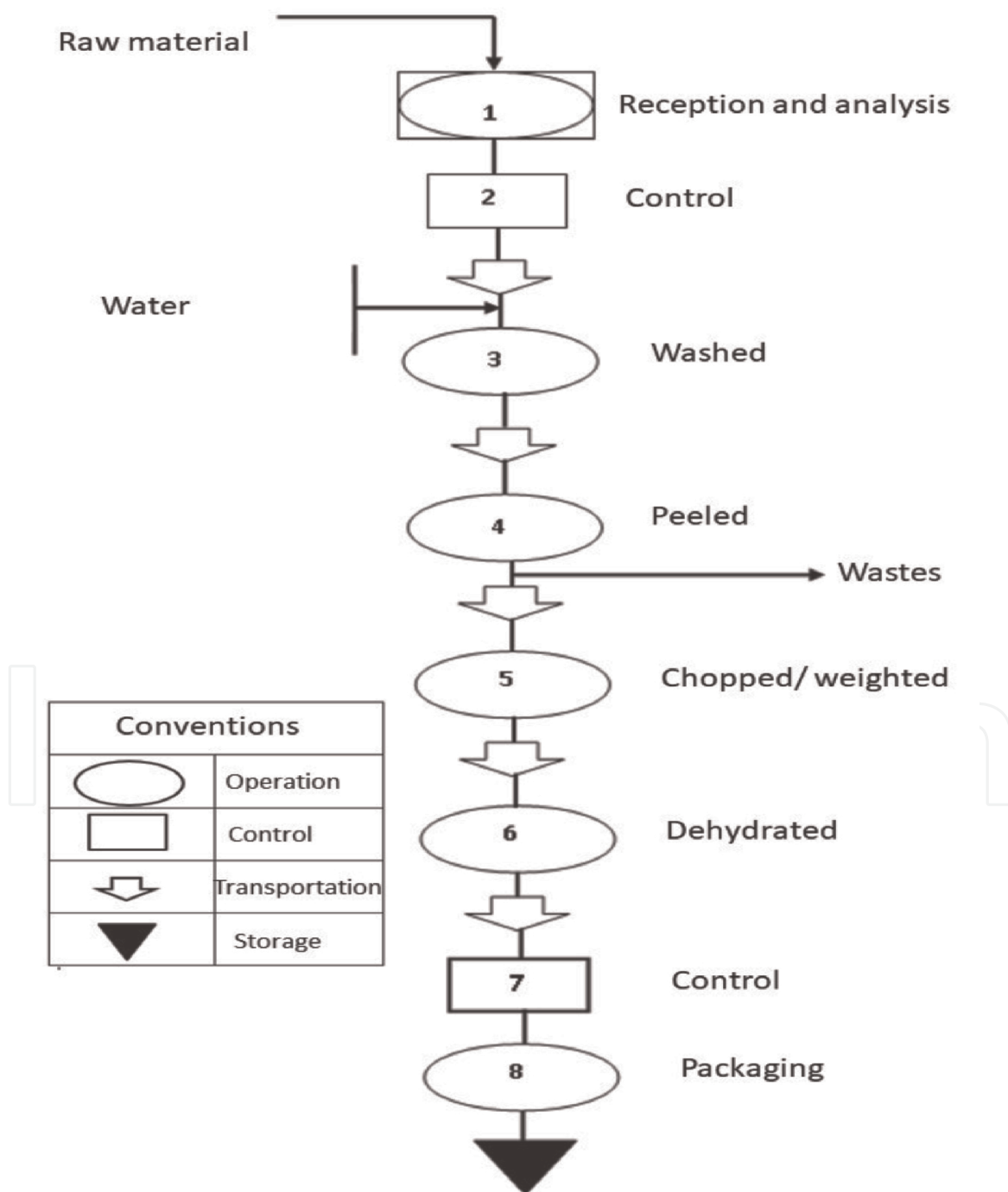
Figure 4. Process flow chart of dried pineapple, mamey, and banana fruits.
