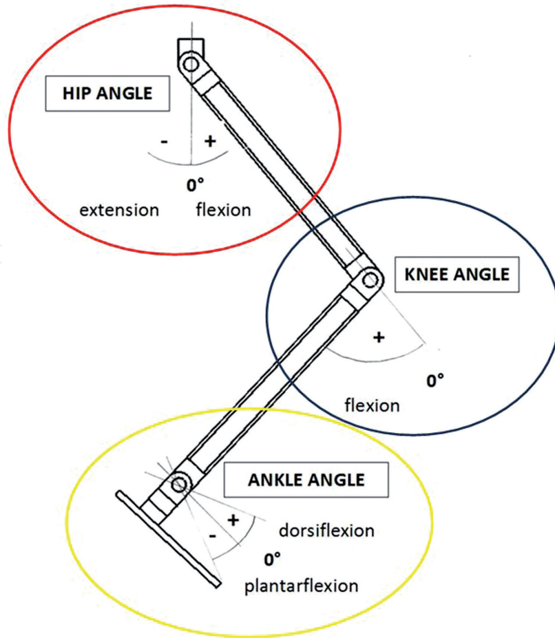
Figure 6. P.I.G.R.O. main reference system.
