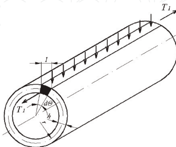
Figure 1. Geometry of circular cylindrical plate structure.
