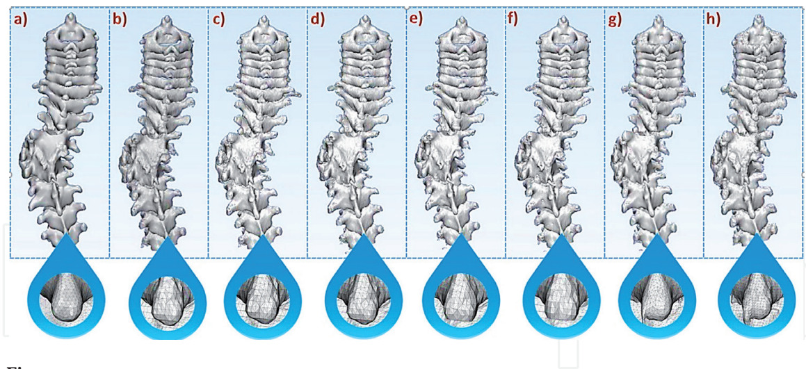
Figure 2. Reference model and each generated 3D test model with a local mesh view (a) Reference model, (b) Binomial blur filter in MIMICS, (c) Curvature flow filter in MIMICS, (d) Discrete gaussian filter in MIMICS, (e) Mean filter in MIMICS, (f) Median filter in MIMICS, (g) Smooth function in 3-Matic and (h) Wrap function in 3-Matic.
