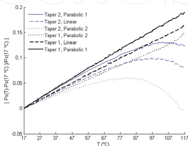
Figure 6. Normalized amplified signal for different temperatures at the end of the tapered fiber with L = 3\text{ m} .
