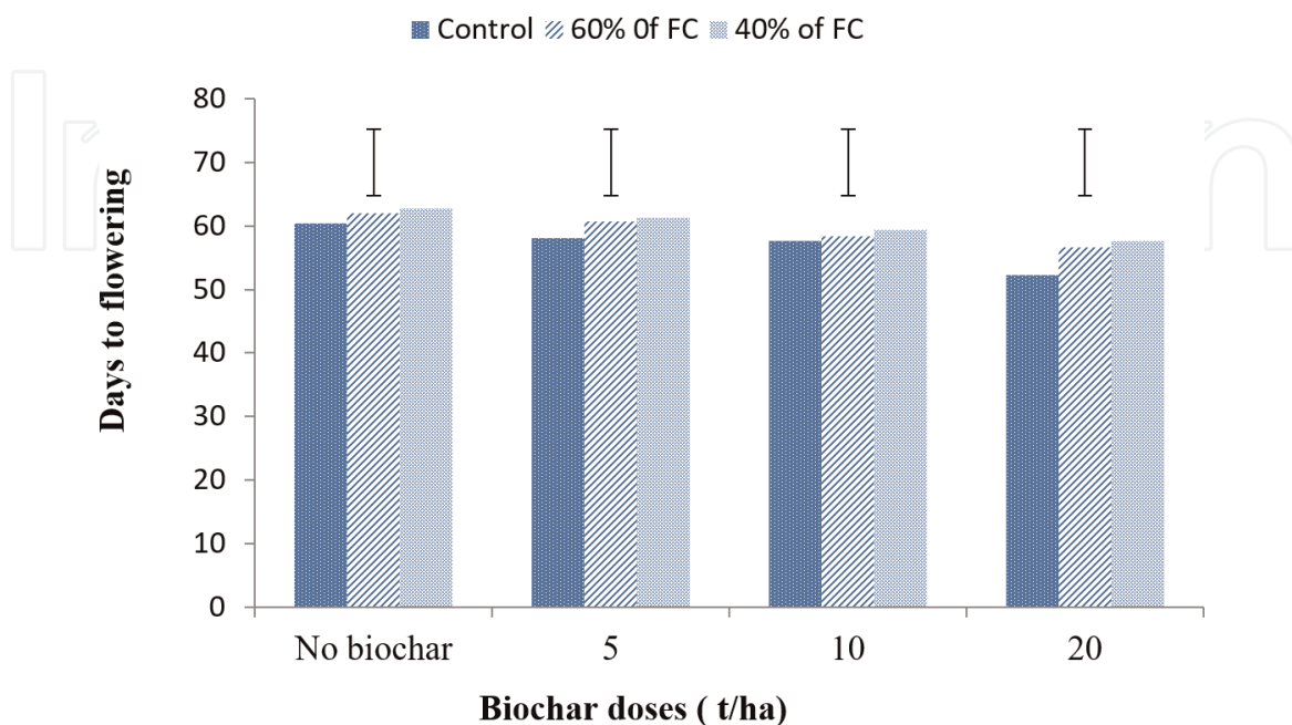
Figure 1. Effect of rice husk biochar on days to flowering of maize under drought conditions. Bar indicates LSD at 5% level of significance.
