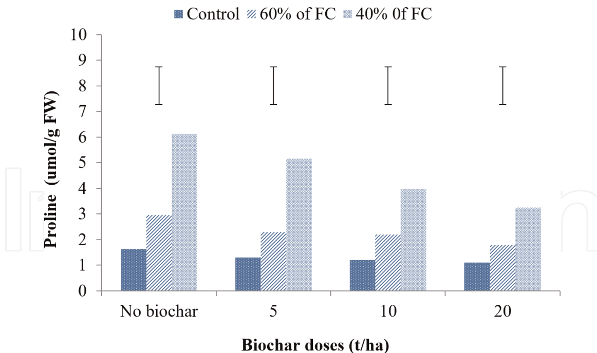
Figure 4. Effect of rice husk biochar on proline content of maize under drought conditions. Bar indicates LSD at 5% level of significance.
