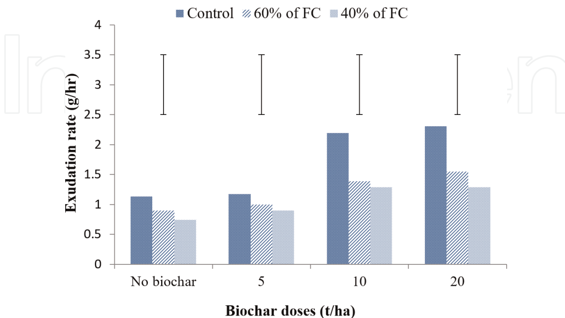
Figure 3. Effect of rice husk biochar on exudation rate of maize under drought conditions. Bar indicates LSD at 5% level of significance.
