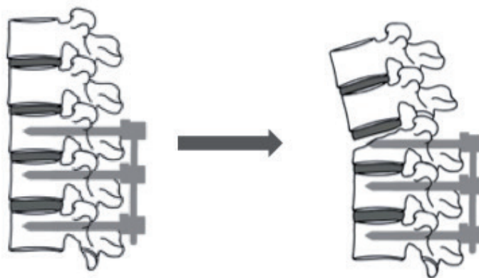
Figure 5. Type 3 failure (endplate failure).
