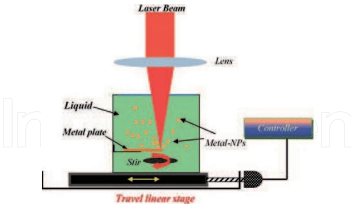
Figure 4. Laser ablation setup [43].
