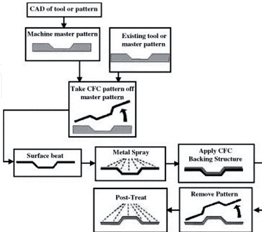
Figure 2. Spray metal tooling [7].
