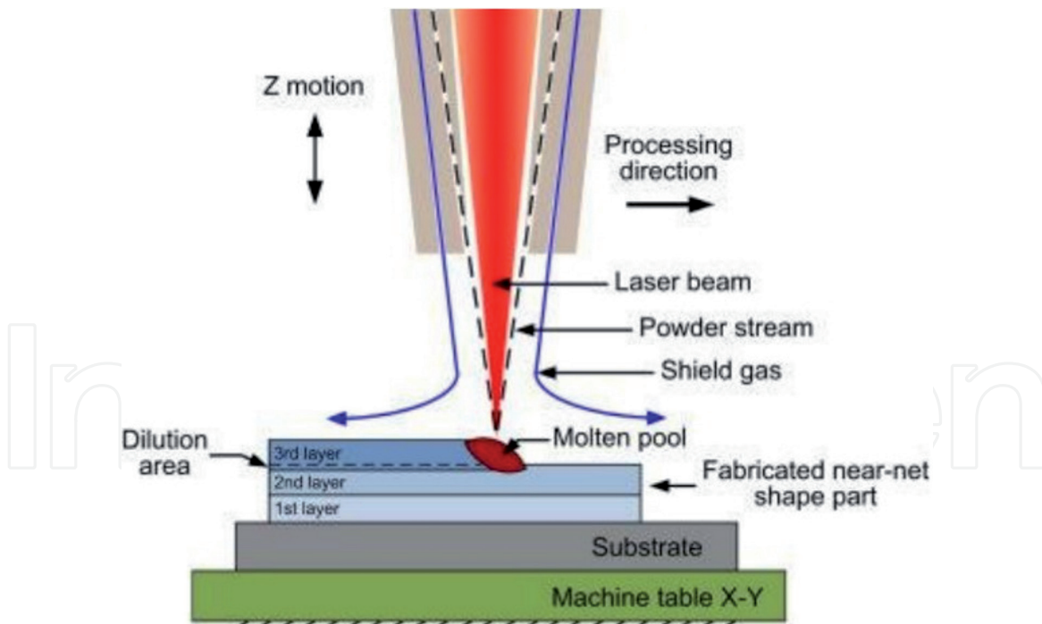
Figure 6. Laser-engineered net shaping (LENS) process [11].
