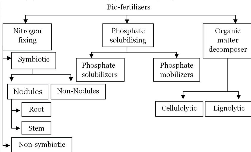
Figure 1. A broad classification of biofertilizers.
