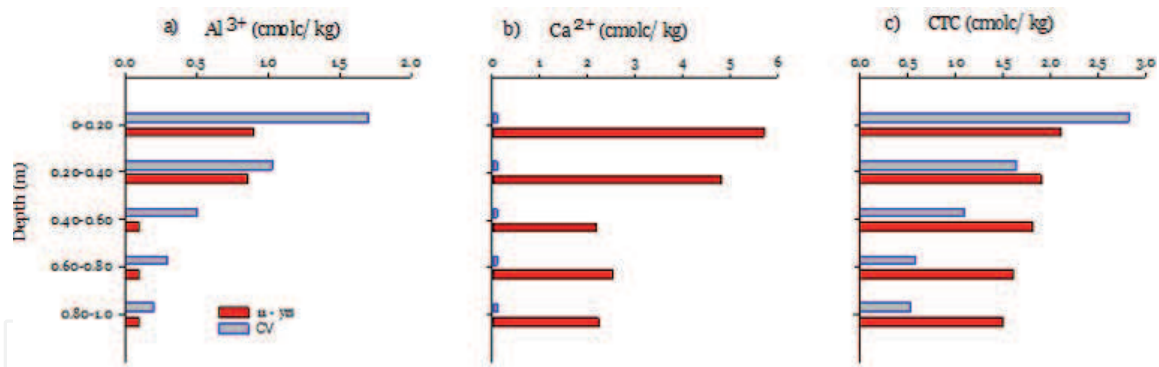
Figure 1. Contents of Al^{3+} (a), Ca^{2+} (b) and effective CEC (c) in red Latosol under conventional management and after 11 years of deep preparation conservation system and application of 28 \text{ Mg ha}^{-1} of gypsum. Source: From authors.
