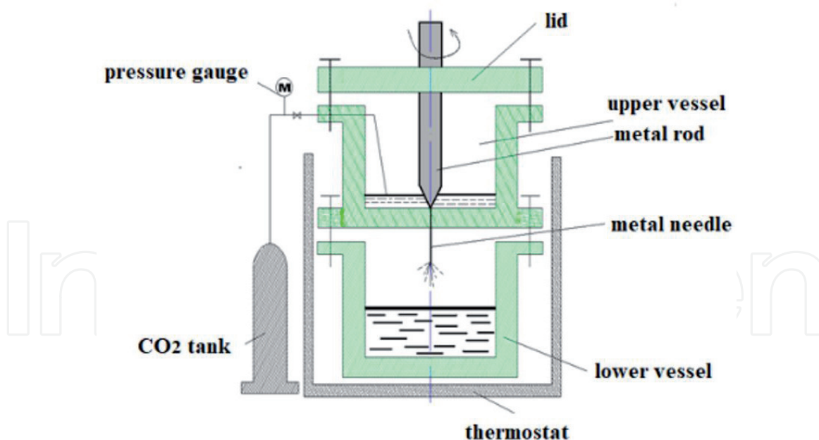
Figure 2. Experimental setup for RESS technique.
