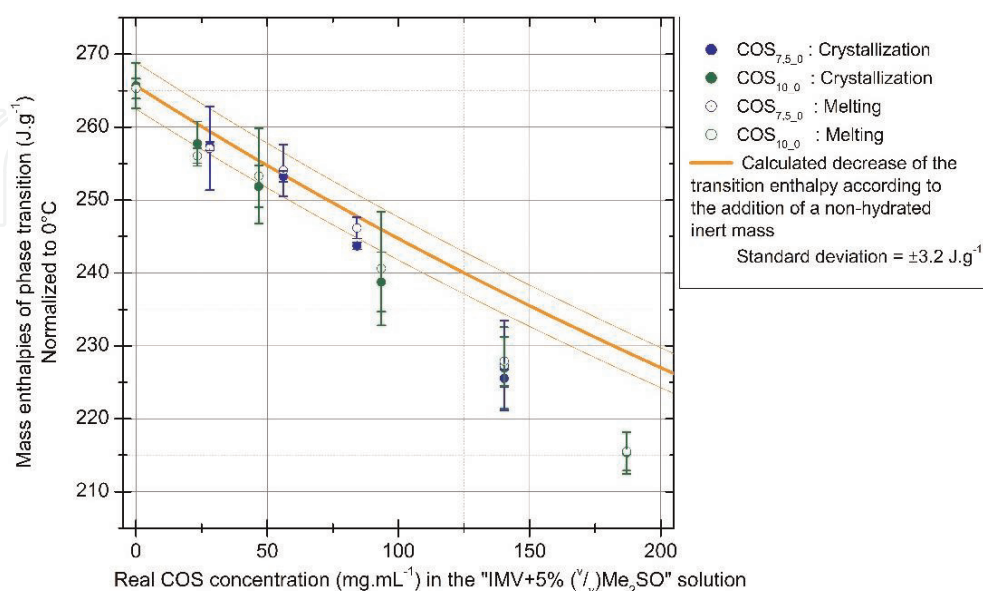
Figure 1. Crystallization and melting enthalpies, normalized to 0^{\circ}\text{C} , for the different solutions containing COS. Here the calculated transition enthalpies are also materialized in the case of the addition of a non-hydrated inert mass in solution. The standard deviations are calculated according to the three data obtained for each value. The standard deviation of the calculated enthalpy is the standard deviation of the measured value without COS.
