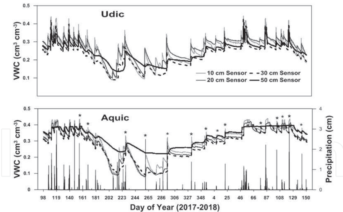
Figure 5. Volumetric water content and precipitation over time with depth (10, 20, 30, and 50 cm) for the udic and aquic inter-mound. Precipitation events denoted with an asterisk were used for statistical analysis.
