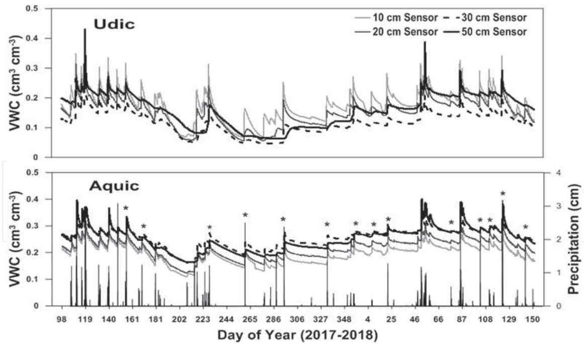
Figure 4. Volumetric water content and precipitation over time with depth (10, 20, 30, and 50 cm) for the udic and aquic mound summit. Precipitation events denoted with an asterisk were used for statistical analysis.
