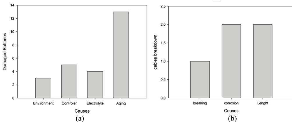
Figure 13. (a) Damaged batteries and their causes and (b) cables breakdown versus causes.
