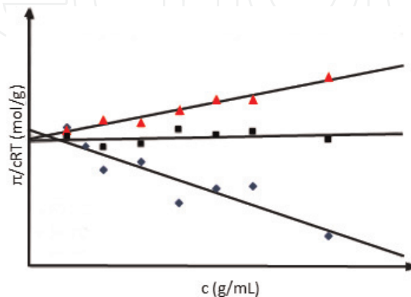
Figure 5. Obtaining M_n through osmometry, the value at zero concentration is extrapolated from the experimental measurements.
