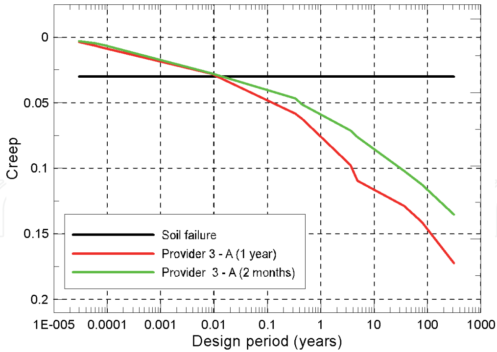
Figure 7. Behavior according to environmental exposure time (Neoloy®).
