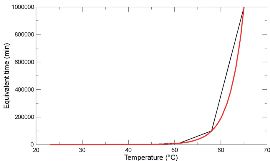
Figure 5. Time-temperature superposition.
