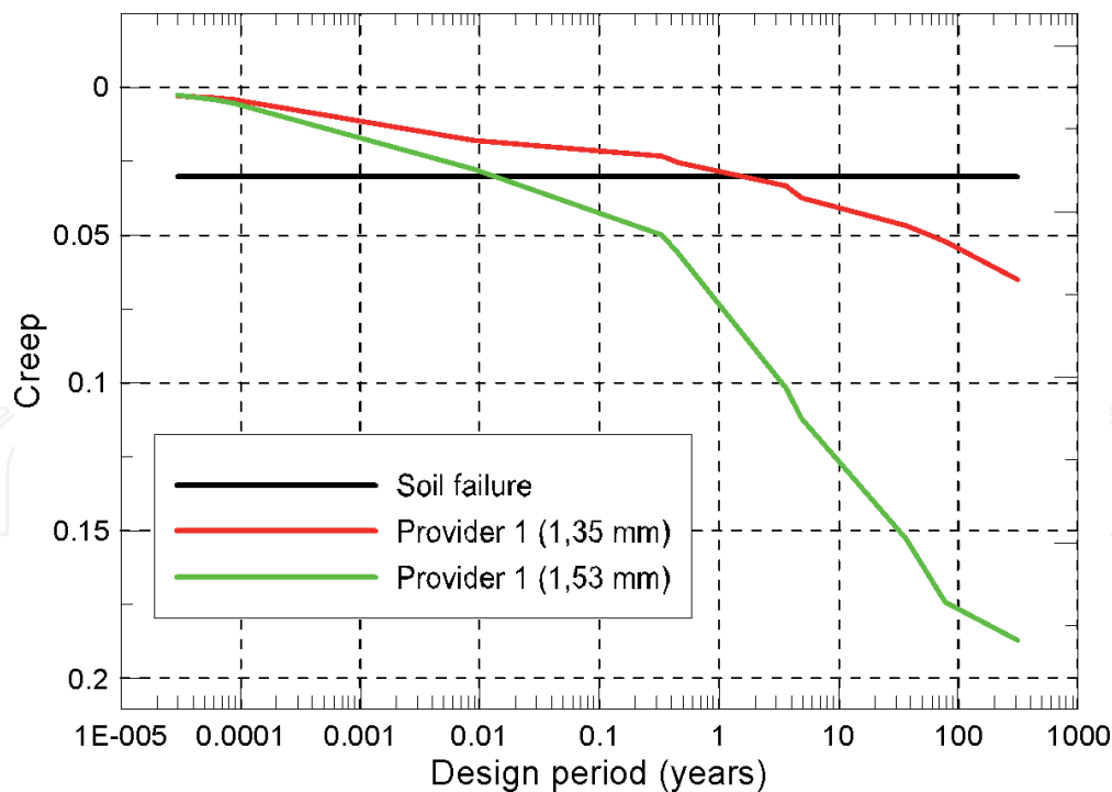
Figure 9. Behavior HDPE geocells according to thickness.
