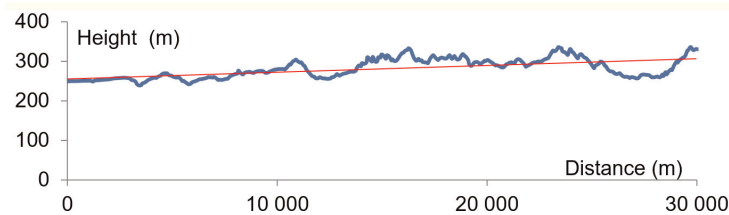
Figure 5. Airport terrain profile with straight line fitting.
