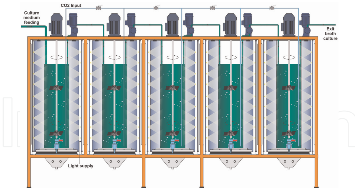
Figure 3. Schematic representation of a series of photobioreactors to operate in continuous cultivation to produce fine chemicals.
