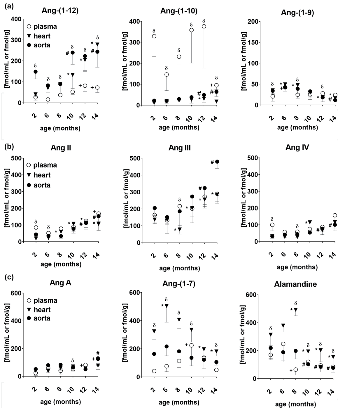
Figure 3. Angiotensin profile in plasma, the heart, and the aorta in Tgaaq*44 mice. Concentration of Ang-(1-12), Ang-(1-10), and Ang-(1-9) (a), Ang II, Ang III and Ang IV (b), Ang A, Ang-(1-7), and alamandine (c) in plasma, aorta, and heart homogenates. * P < 0.05 for the heart tissue of a given group of Tgaaq*44 mice vs. 2-month-old Tgaaq*44 mice; # P < 0.05 for the aorta tissue of a given Tgaaq*44 group vs. 2-month-old Tgaaq*44 mice; + P < 0.05 for plasma of a given Tgaaq*44 group vs. 2-month-old Tgaaq*44 mice (one-way ANOVA with Tukey post hoc test or Kruskal-Wallis); \delta P < 0.05 hearts vs. plasma ( t -test or Wilcoxon test). Reprinted with permission from [99].
