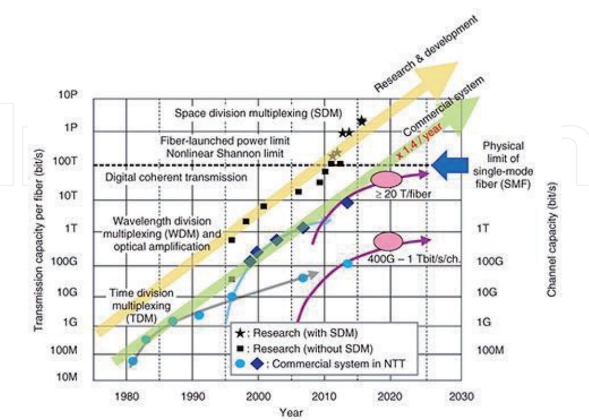
Figure 2. Evolution in optical transmission technology [22].
