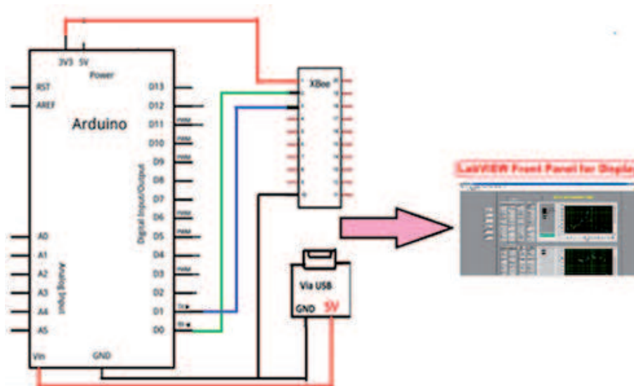
Figure 7. Circuit connection of sink node.
