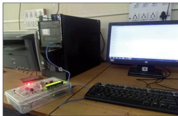
Figure 3. Experimental set up for wired environment monitoring system.
