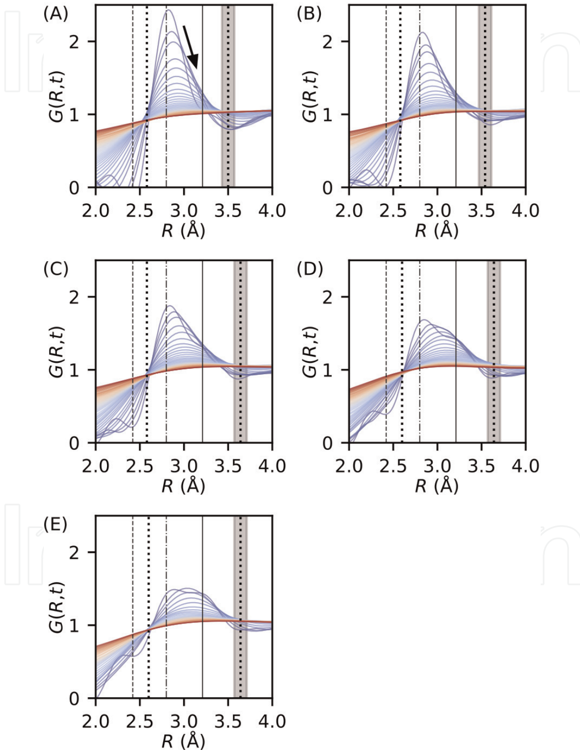
Figure 5. The van Hove functions around the first-neighbor correlation peak, R \sim 2.9 \text{\AA} : (A) pure water, (B) m = 0.75 \text{ mol/kg} , (C) 1.5 \text{ mol/kg} , (D) 2.26 \text{ mol/kg} , and (E) 3.0 \text{ mol/kg} . The solid lines at R = 3.21 \text{\AA} show the R_{O_2^- + R_{Cl^-}} . The dashed line at R = 2.42 \text{\AA} shows the R_{O_2^- + R_{Na^+}} . The dash-dotted line at R = 2.8 \text{\AA} shows the R_{O_2^- + R_{O_2^-}} . The range between the dotted lines ( R_1' and R_1'' ) was used to calculate the area, A(t) , of the first neighbor. The upper limit of this range is changed within the gray-shaded area to estimate the uncertainties [25].
