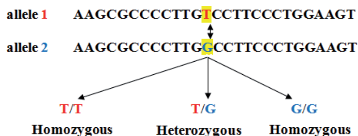
Figure 5. Single nucleotide polymorphism for two alleles.
