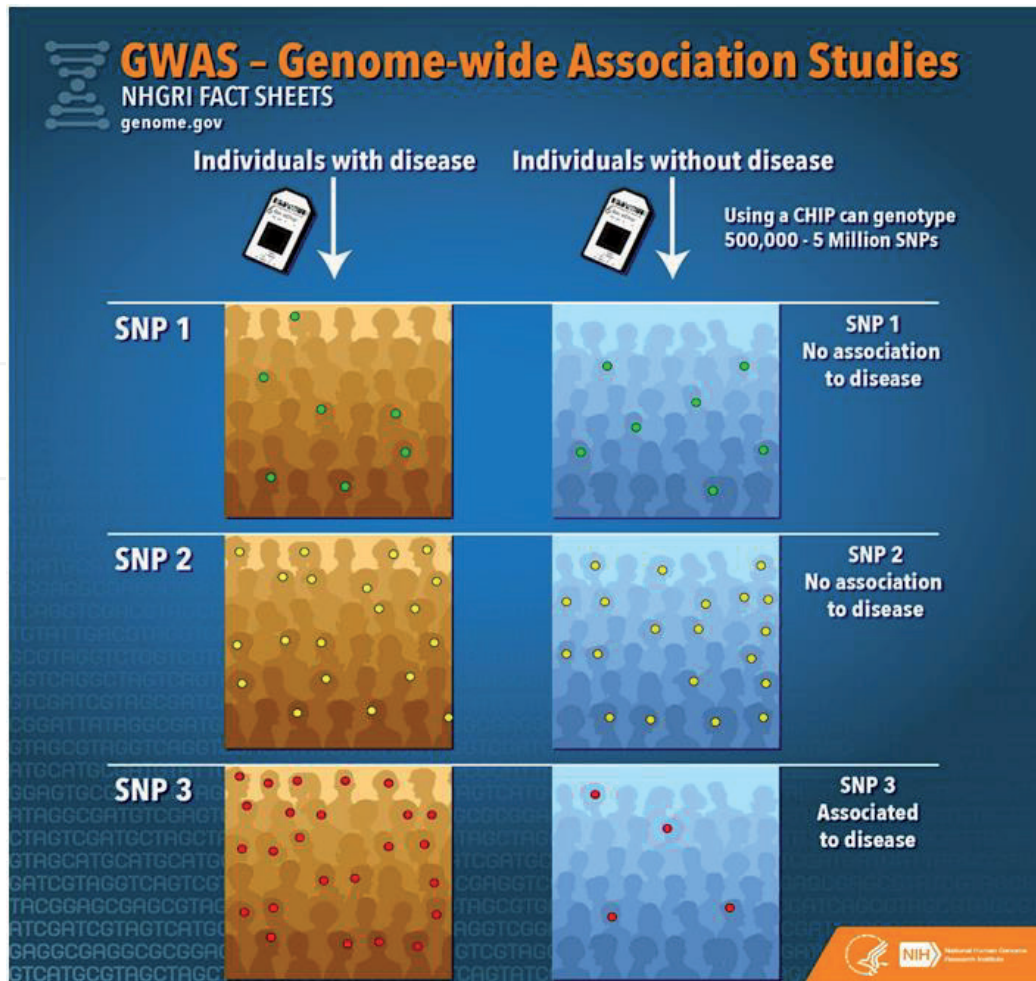
Figure 6. Genome-wide association studies [71].
