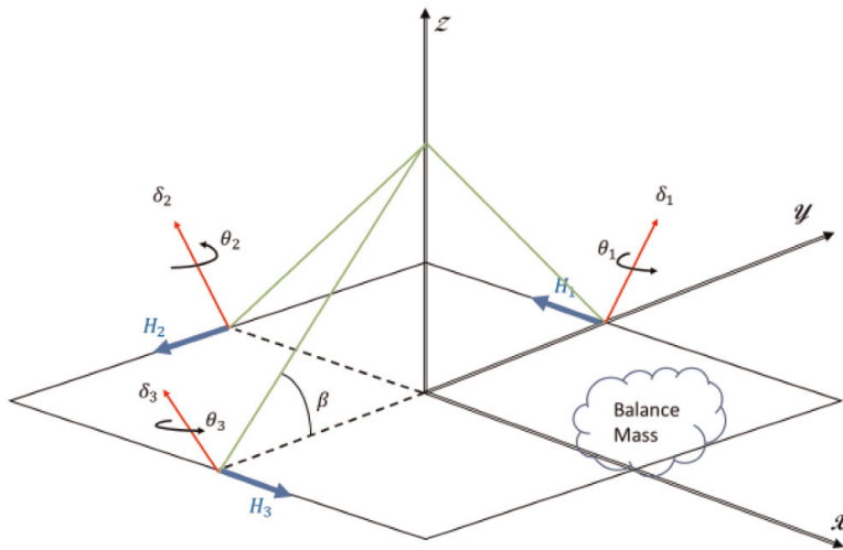
Figure 2. 3/4 configuration of CMGs on a spacecraft.
