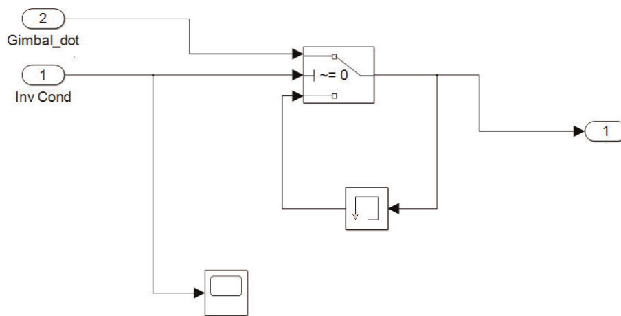
Figure 3. Singularity penetration with unit delay logic.
