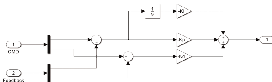
Figure 4. PDI controller topography.
