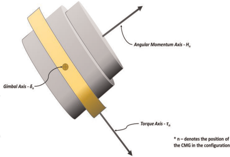
Figure 1. CMG angular momentum-torque-gimbal axis representation.
