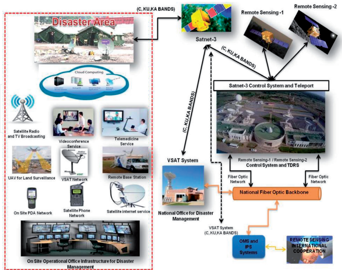
Figure 11. Emergency communications network topology for disaster events management.
