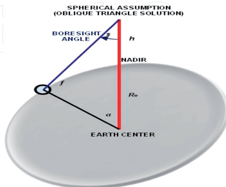
Figure 4. Oblique spherical triangle method to predict the remote sensing sensor potential terrain swath coverage in nadir angle and off-nadir angle ( RSTSC_p ).
