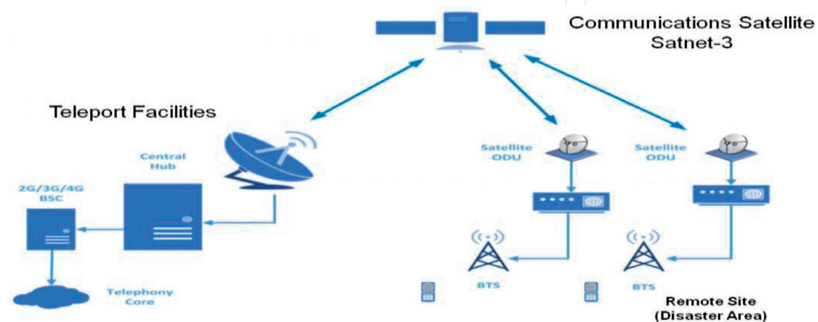
Figure 10. Technology solutions for disasters management cellular backhaul-SCPC over satellite.
