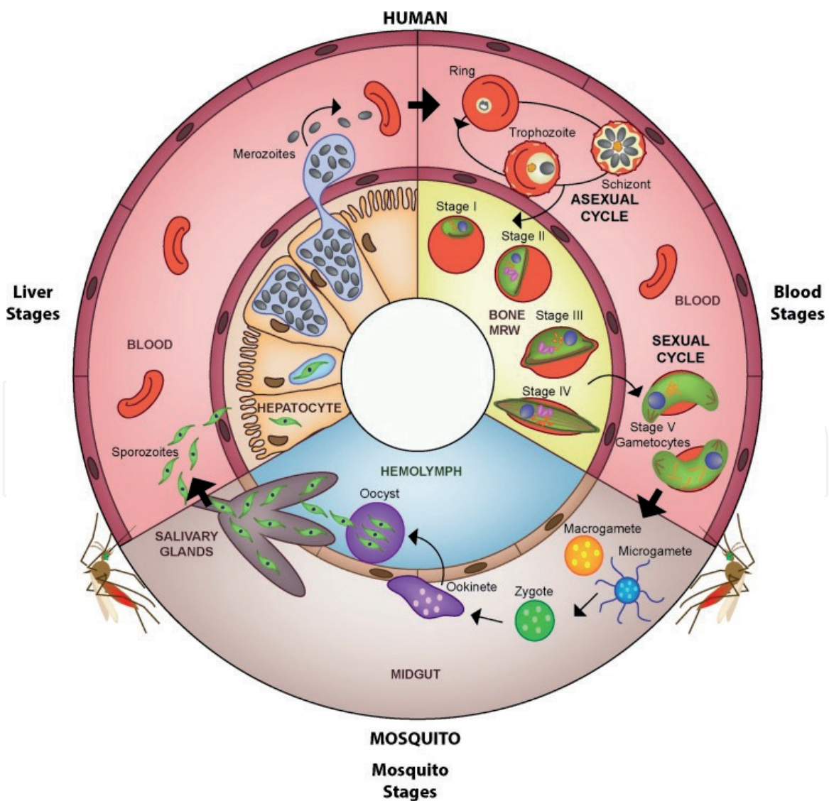
Figure 1. The basic malaria life cycle of Plasmodium falciparum (adapted from [20] with permission).
