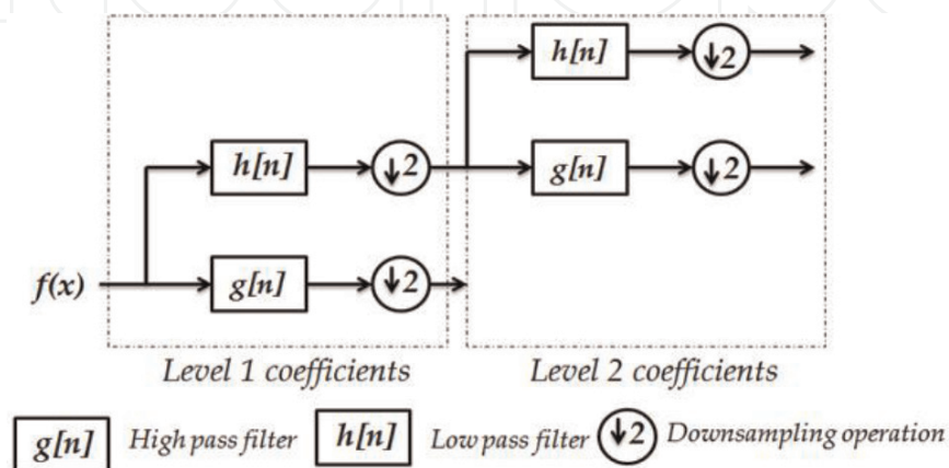
Figure 1. Block diagram of filter analysis.
