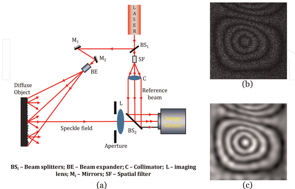
Figure 11. (a) Schematic of DSPI setup [57, 58], (b) Recorded DSPI fringe pattern, and (c) Denoised DSPI fringe pattern by using swt thresholding technique.
