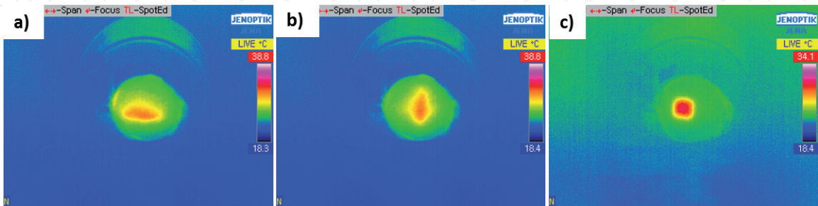
Figure 11. Thermographic camera images during x -axis (a), y -axis (b), and both axes simultaneously (c) sweeping.
