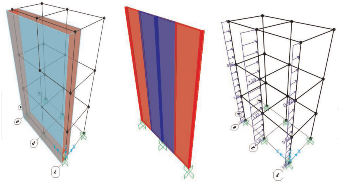
Figure 4. Wind loads on columns.
