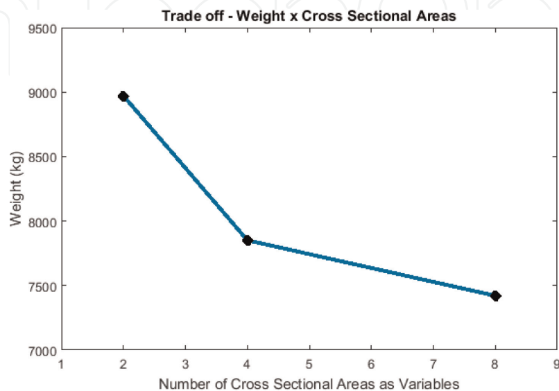
Figure 19. Tradeoff curve of Experiment 3.
