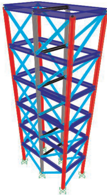
Figure 17. Experiment 4—members linked in five groups according to Table 11.
