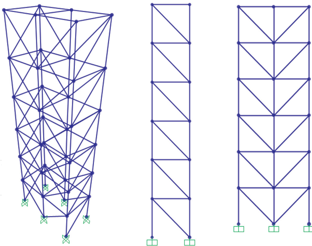
Figure 16. One hundred fourteen members 3D frame—long and short façade.
