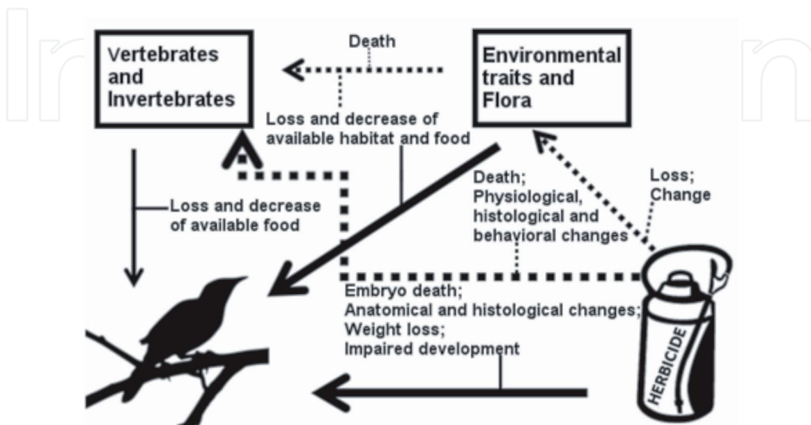
Figure 4. Ecotoxicity of glyphosate-based herbicide (GBH) to aquatic birds. Direct (continuous arrows) and indirect (dashed arrows) effects of GBH on birds.
