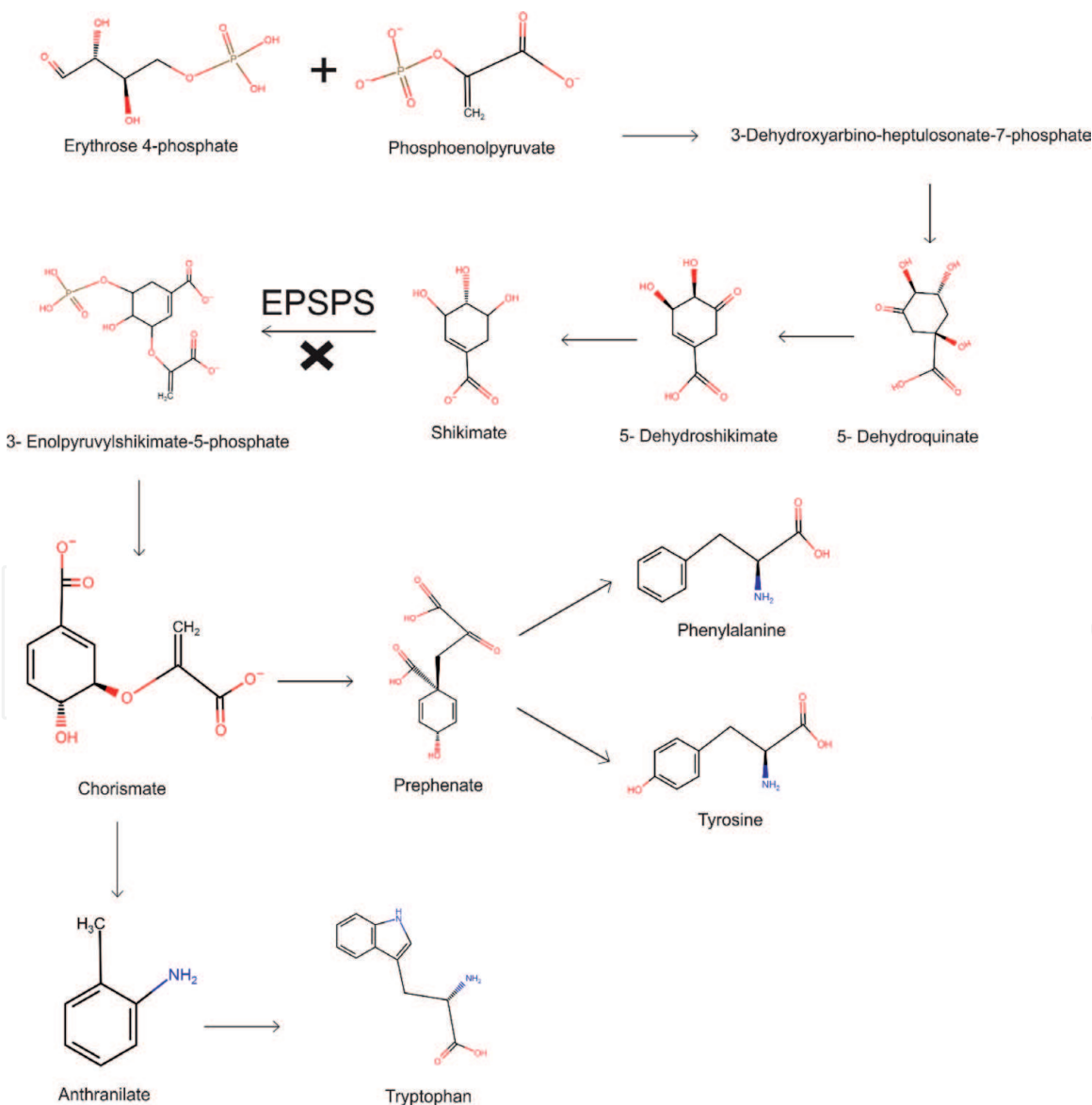
Figure 1. Glyphosate action on the biochemical pathway of plants inhibiting 3-enolpyruvylshikimate 5-phosphate synthase (EPSPS) enzyme and production of essential amino acids as phenylalanine, tyrosine, and tryptophan, causing plant death.
