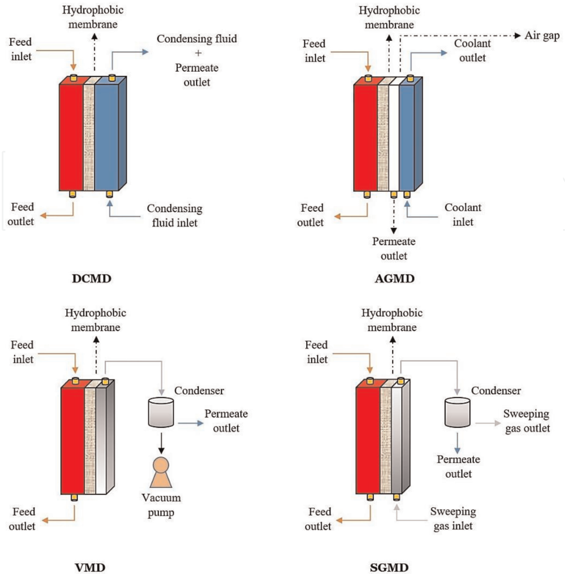
Figure 2. Schematic of various MD configurations.
