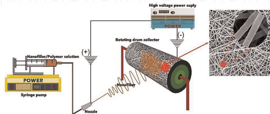
Figure 3. Schematic of electrospinning process. Source: Reprinted from [24].
