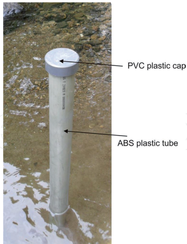
Figure 1. DGT placed in the base of the hollow sampler and left for 24 hours.
