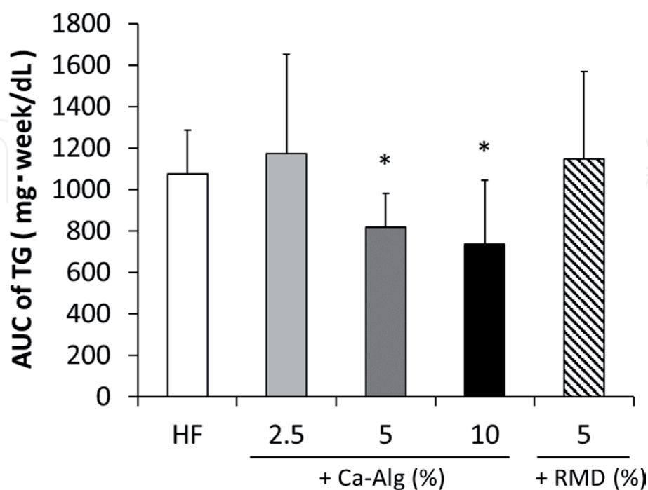
Figure 5. Area under the blood concentration-time curve of TG in rats after the 5-week feeding period with high-fat diet or high-fat diet containing Ca-Alg or high-fat diet containing RMD [24]. The data represent means \pm S.D., n = 7 . p < 0.05 , compared with high-fat diet.
