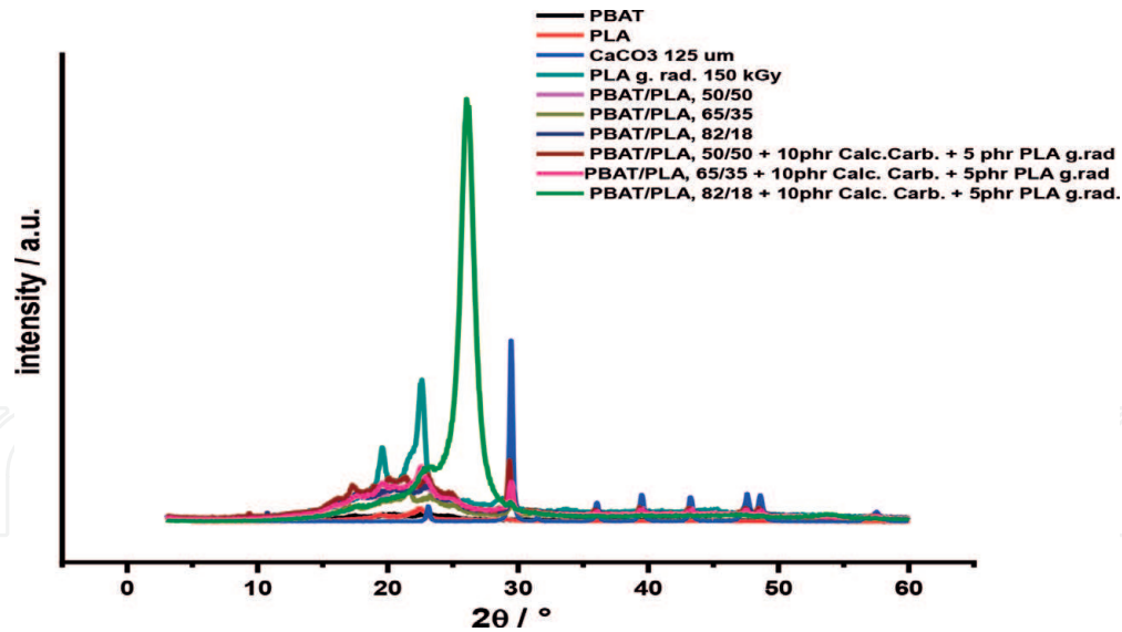
Figure 3. DRX diffractograms of all studied samples.
