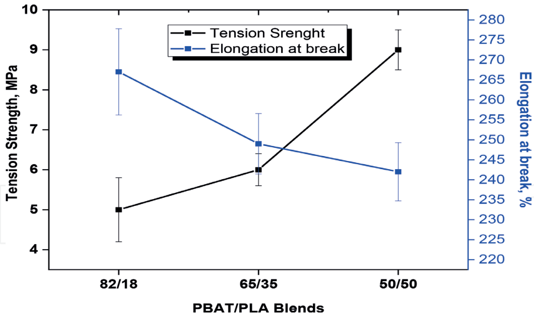
Figure 14. Tensile mechanical properties for PBAT/PLA blends: 82/18, 65/35, and 50/50.
