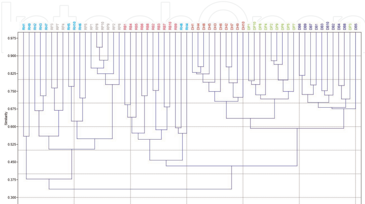
Figure 4. Dendrogram based on the distances of Bray-Curtis from the benthic macroinvertebrate community of the Cunas River, according to sector and sampling season.
