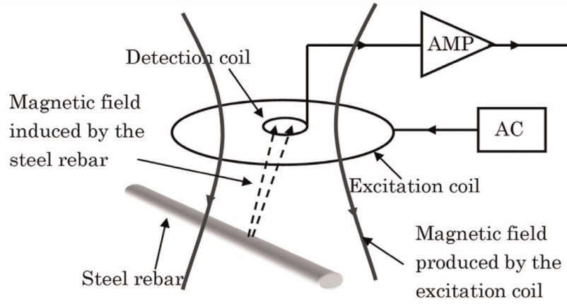
Figure 2. Principle of electromagnetic method.
