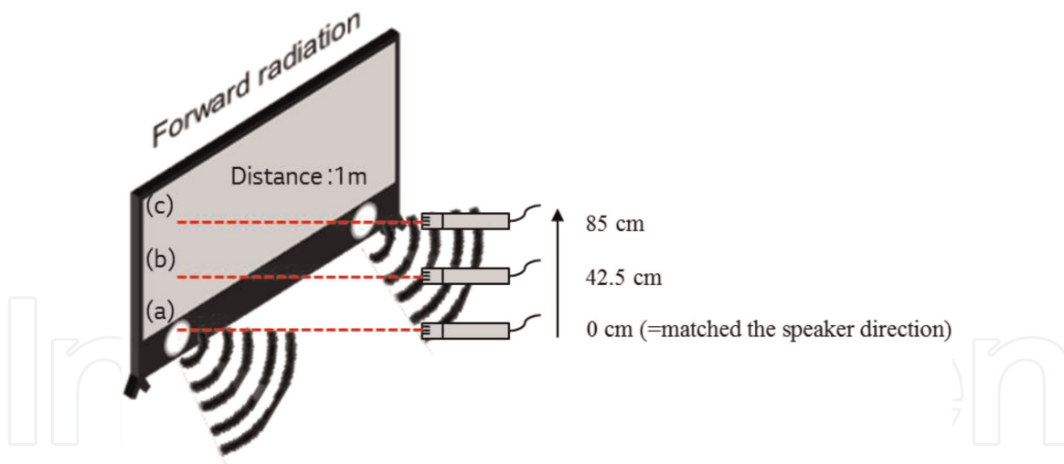
Figure 19. Forward radiation structure, test positions and the distance for the TV sample.
