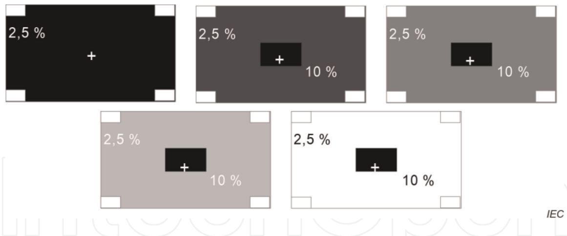
Figure 5. Test patterns for black level and constancy measurement.
