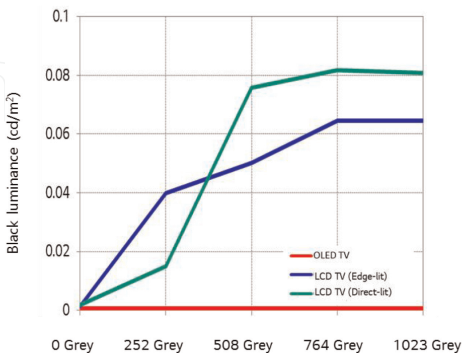
Figure 6. Black luminance according to background grey levels.
