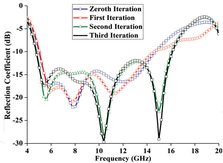
Figure 4. Reflection coefficient of intermediate antenna design steps.
