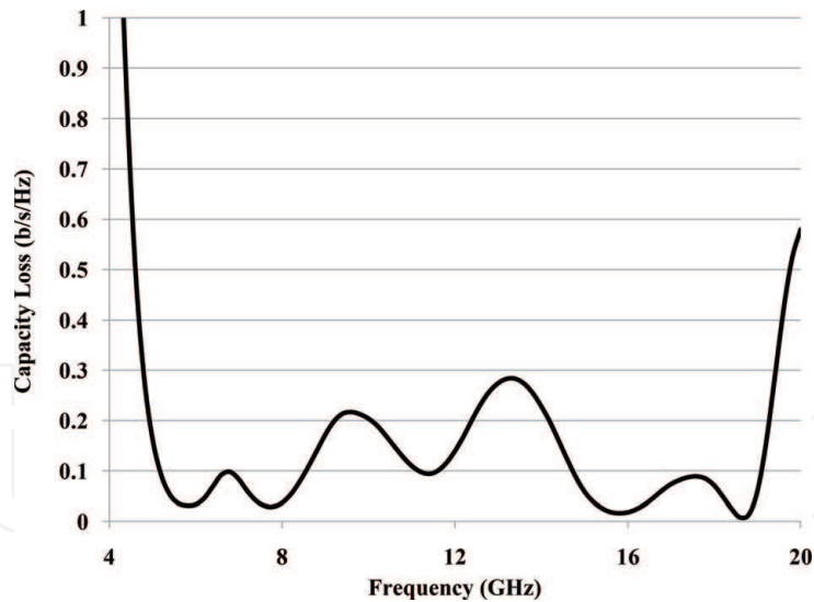
Figure 16. Capacity loss versus frequency characteristic.
