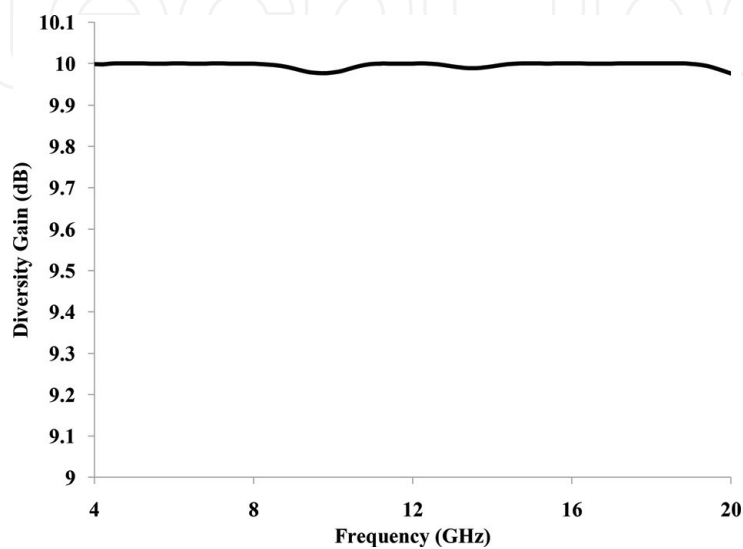
Figure 15. Diversity gain versus frequency characteristic.
