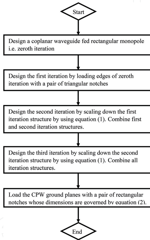
Figure 2. Flow chart of designing initial radiator geometry.
