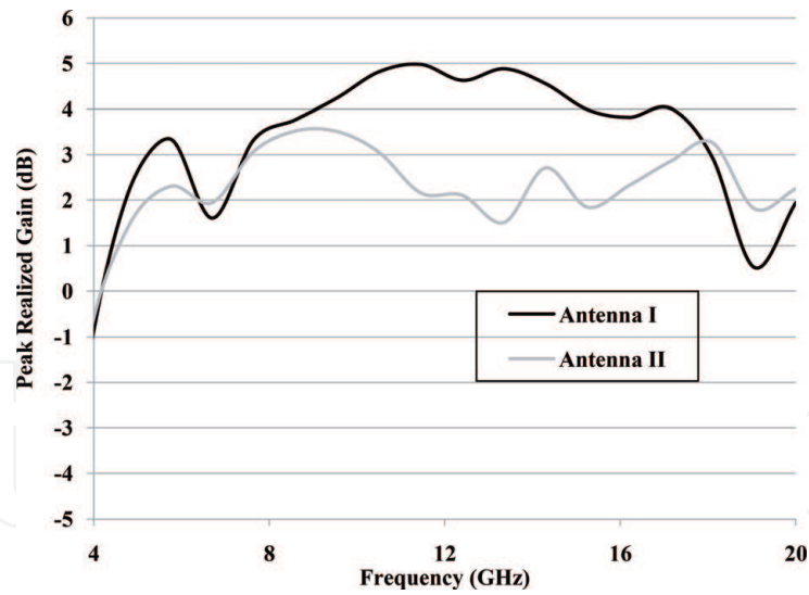
Figure 8. Peak realized gain versus frequency characteristics.
