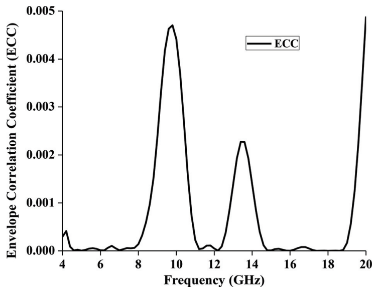
Figure 13. Envelope correlation coefficient versus frequency characteristic.
