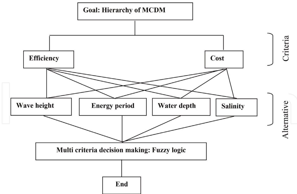
Figure 2. Figure showing the hierarchy of the MCDM methodologies.
