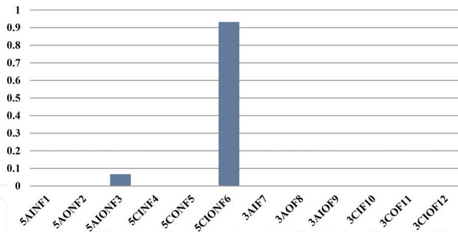
Figure 4. The 12 models developed for prediction of suitable site selection.
